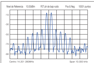
14MHz transmit IMD example (100W output)
